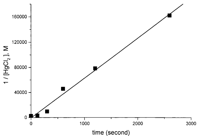
Figure 2. Second order kinetic plot for sorption of mercury from 100 mL \text{HgCl}_2 solution (initial concentration 3.7 \times 10^{-4} M) while contacting with 0.2 g. of polymer sample.
