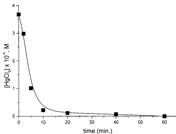
Figure 1. Concentration-time plot of 100 mL \text{HgCl}_2 solution (initial concentration 3.7 \times 10^{-4} M) while contacting with 0.2 g. of polymer sample.
